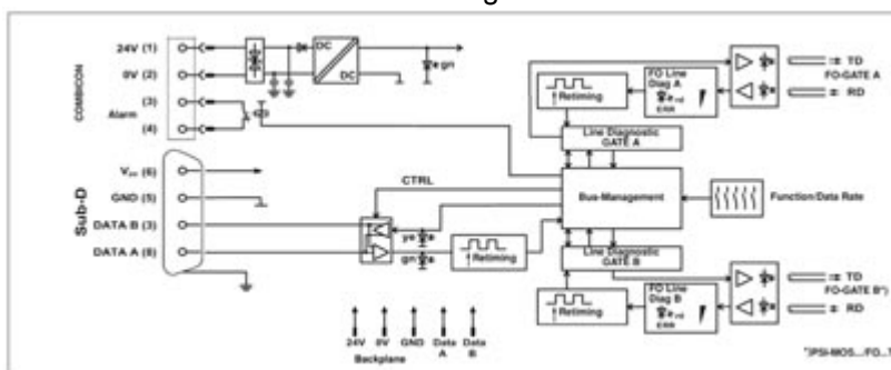
Block diagram
